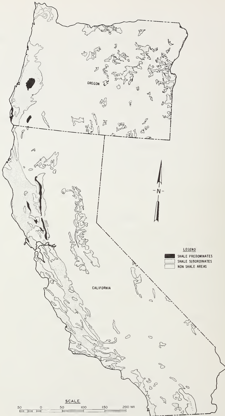
Figure 2. Shale occurrence; Oregon and California.
